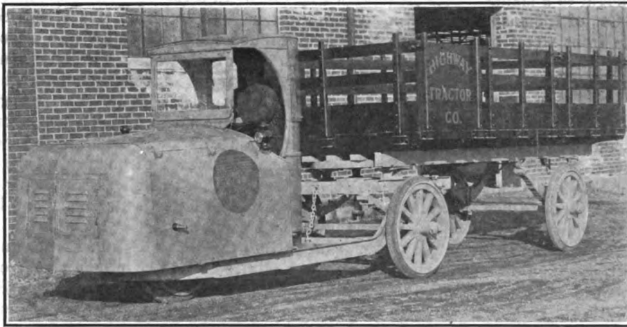
Truكتور coupled to a 6,000 lb. semi-trailer unit on rubber tired wheels, ready for driving straight ahead
